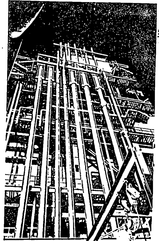
Public Service Company of Oklahoma Station at Tulsa.
