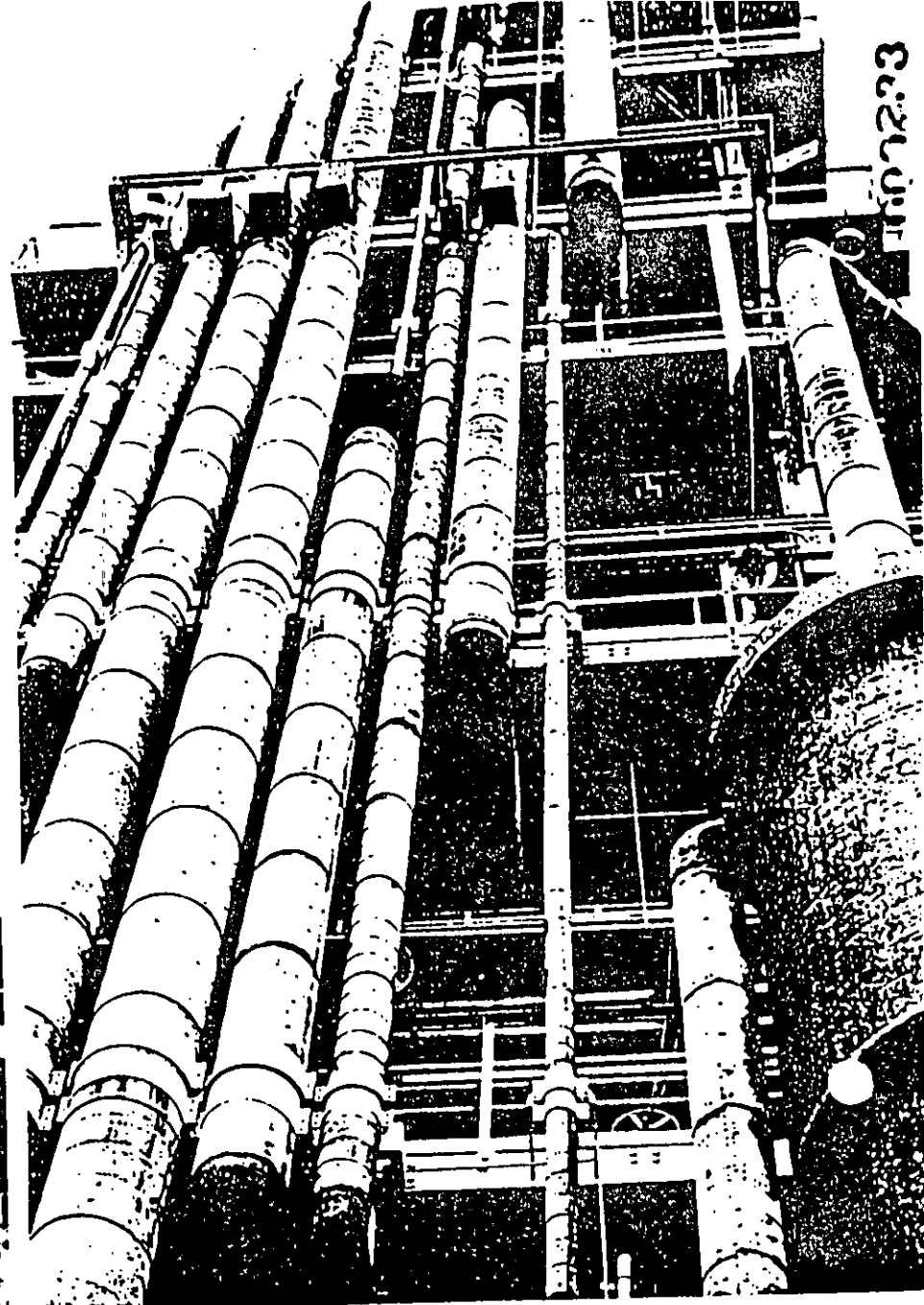
Ethylene Plant of Monsanto Chemical Company at Texas City, Texas.
