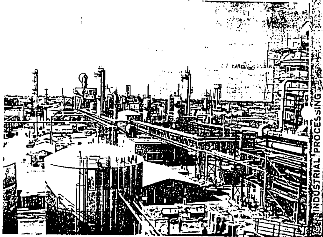
Hopewell, Virginia Plant of National Aniline Division of Allied Chemical Corporation.
